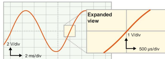
Figure 12B. Sinusoid waveform comparison at 100 Hz (B2961B/B2962B)
