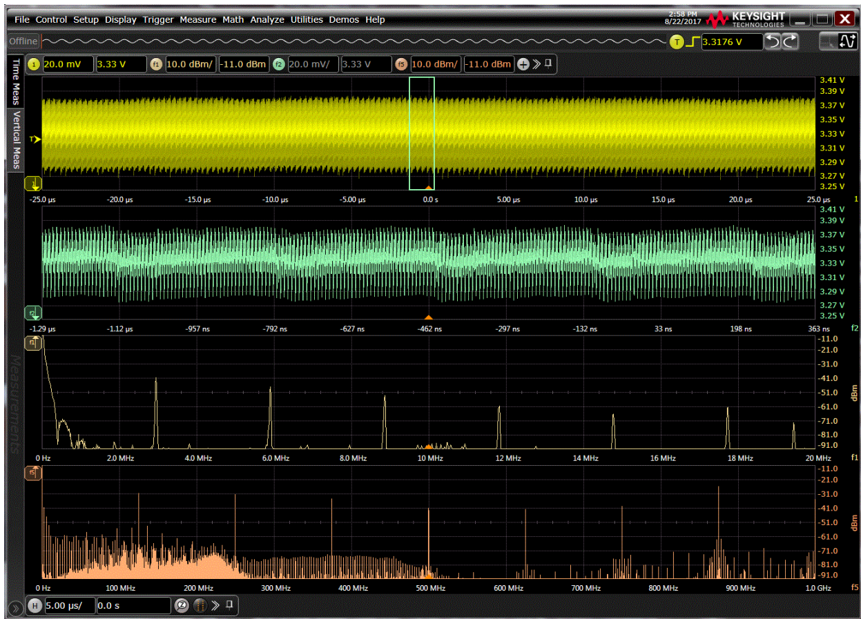
Figure 22. N7020A Power Rail Probe and S-Series High-definition oscilloscope measuring the noise on a 3.3 V supply.
