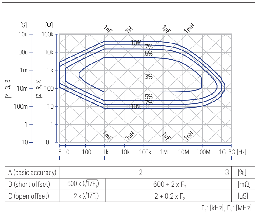
Figure 3. Impedance measurement accuracy (SPD), S-parameter port 1-2 series-thru method.
