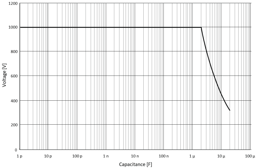
Figure 14. Maximum discharge withstands voltage (typical)
