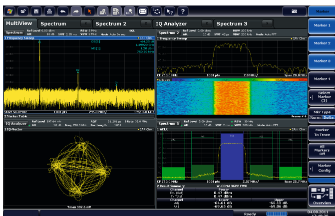
MultiView function.
