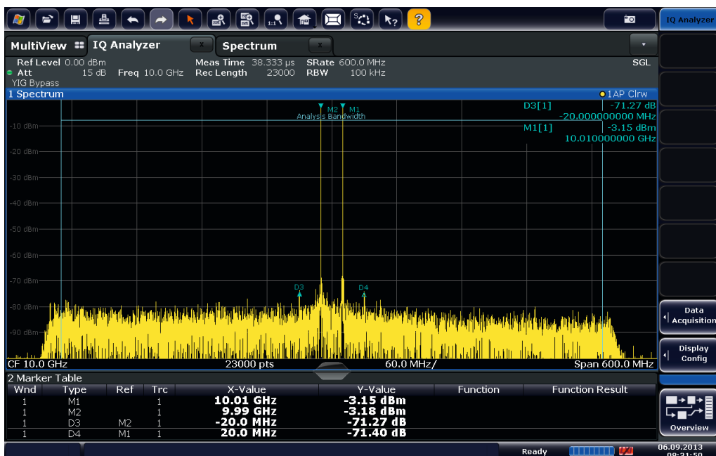
Third-order intermodulation distortion (IM3) of -65 dBc, measured with the R&S®FSW-B500 option.
