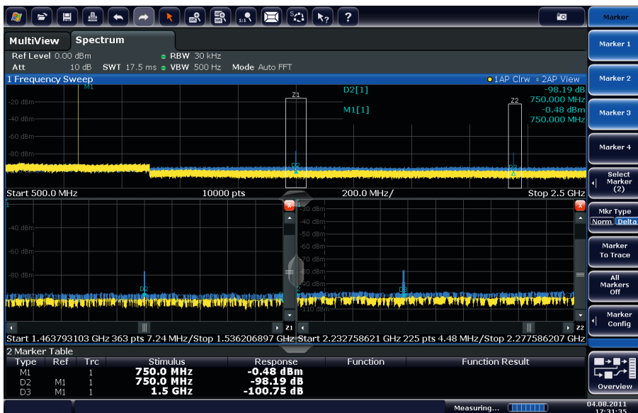
Harmonic measurement with highpass filter on (yellow trace) and off (blue trace).
