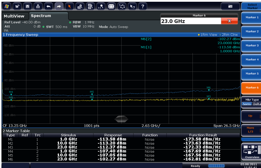
Displayed average noise level (DANL) with preamplifier and noise cancellation switched on.
