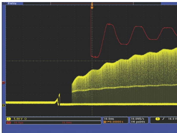
Modulation analysis on an IGBT's gate drive during power-up
